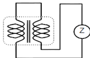
Differential Mode
