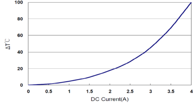
WLPSMD201210FR47M-S
