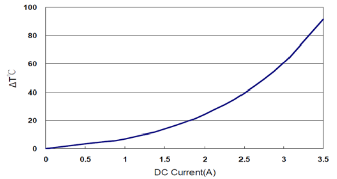
WLPSMD201210FR68M-S
