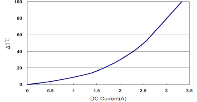
WLPSMD201210F1R0M-S
