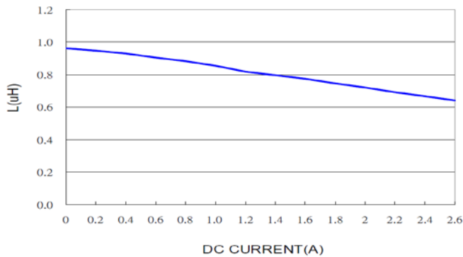
WLPSMD201210F1R0M-S
