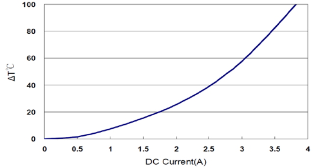
WLPSMD201210FR33M-S
